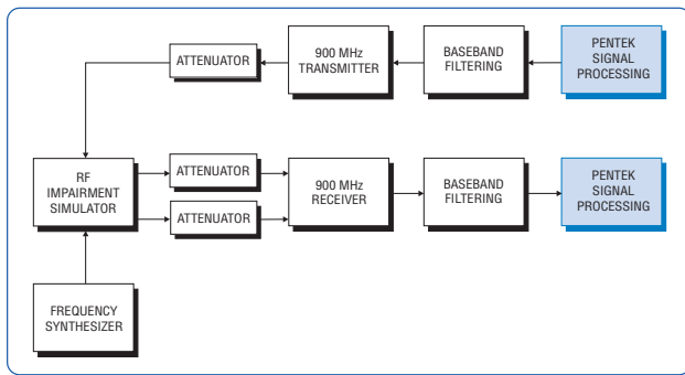
Figure 4. Hardware Configuration for Measurements
