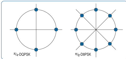
Figure 2. Constellation Diagrams (after demodulation)
