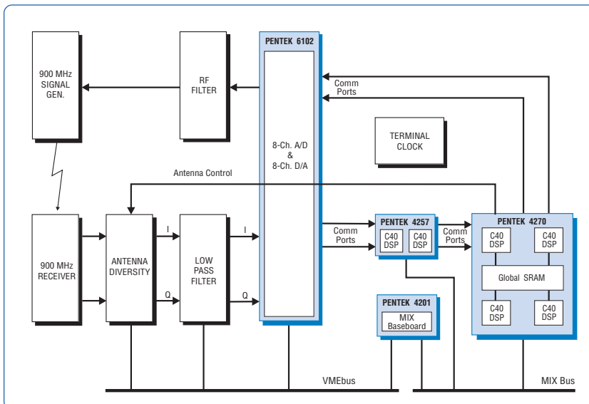
Figure 3. Signal Processing Downlink System Block Diagram
